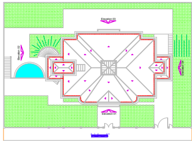
Roof Plan
