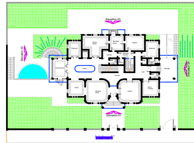
First Floor Plan A = 367,78 m 2
