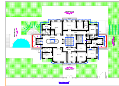
Second Floor Plan A = 330,41 m 2
